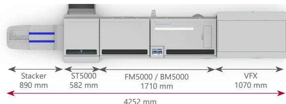
BM5000 System with ST5000 - Machine footprint
