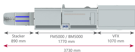
BM5000 System with VFX feeder - Machine footprint
