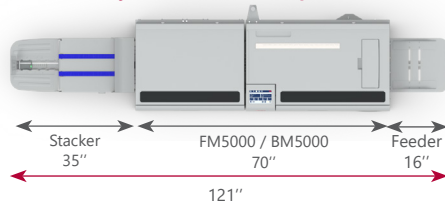
BM5000 System with CST5000 - Machine footprint
