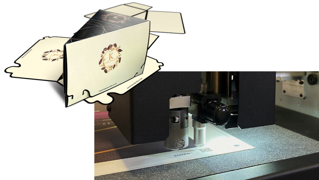
Dual tool head for rapid cut and crease includes tangential crease capability
