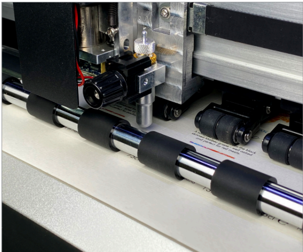
Blade holder offers blade changes dependent on media type
