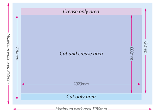
Diagram showing media, cutting and creasing areas with overlap common areas for both
