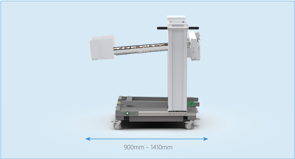
MPS XL - Machine footprint
